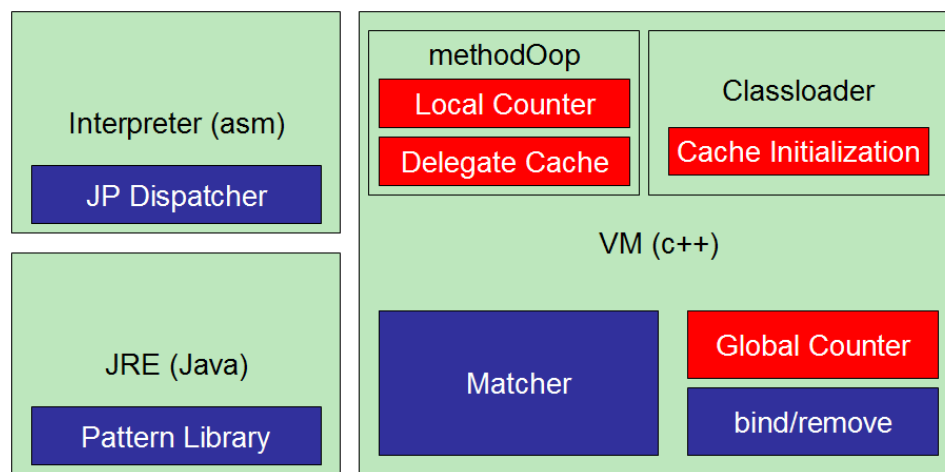
Figure 3.1 Overview of Nu 's VM Implementation
