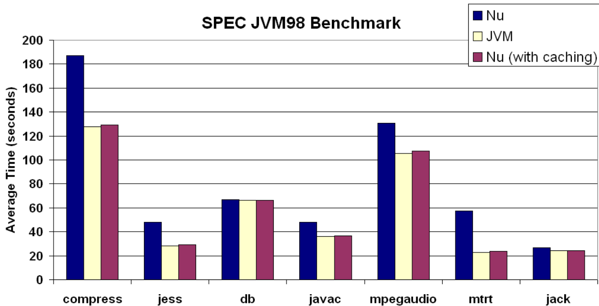
Figure 5.2 Comparison of Join Point Dispatch Times Using the SPEC JVM98 Benchmark (smaller bars are better)
