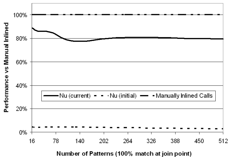
Figure 5.3 Invoke Benchmark - Varying Number of Patterns
